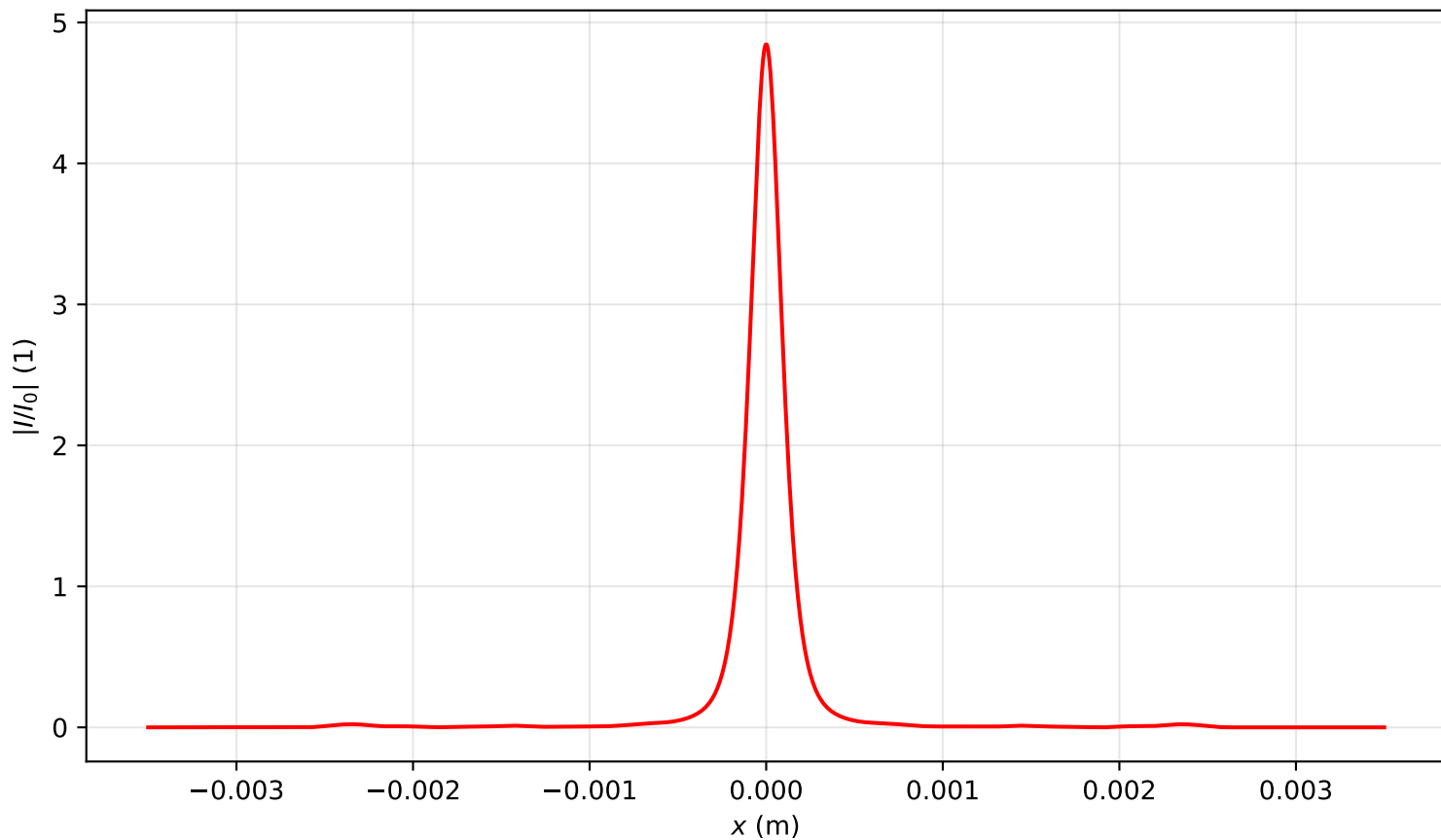
Intensity profile I(x, y = 0, z = 3.582)/I_0 , \text{Pin}=2.5\text{Pcr} , artificial time
